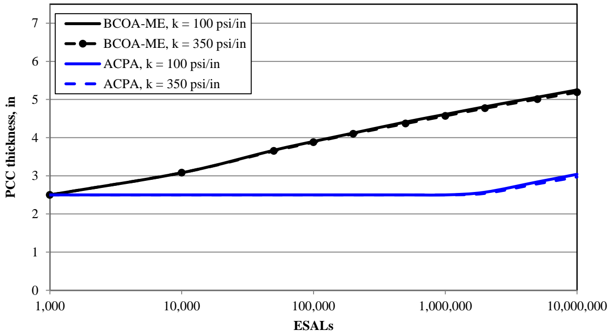
Figure 15. PCC thickness sensitivity to k value for 4 ft × 4 ft slabs with respect to design ESALs
