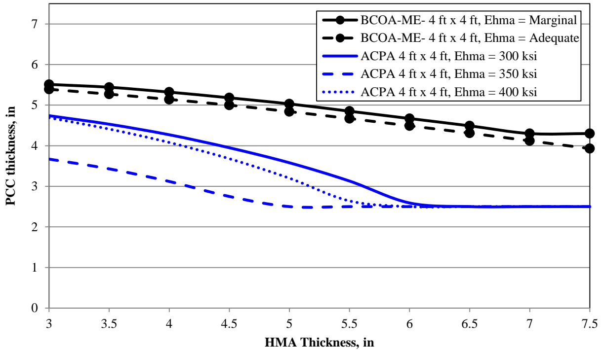
Figure 10. PCC thickness sensitivity to HMA quality for 4 ft × 4 ft slabs with respect to HMA thickness
