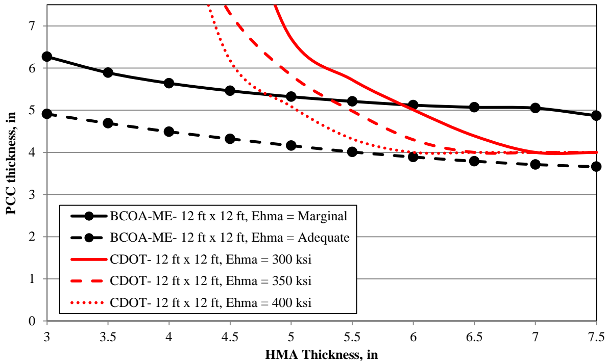
Figure 13. PCC thickness sensitivity to HMA quality for 12 ft × 12 ft slabs with respect to HMA thickness
