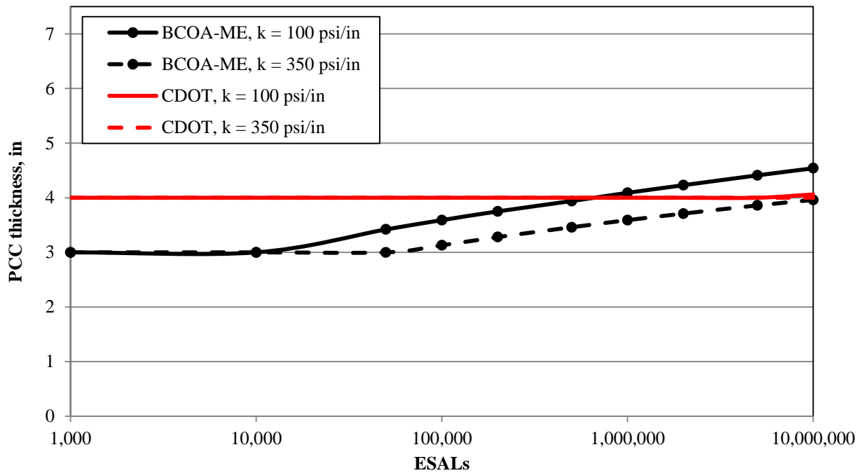
Figure 16. PCC thickness sensitivity to k value for 6 ft × 6 ft slabs with respect to design ESALs
