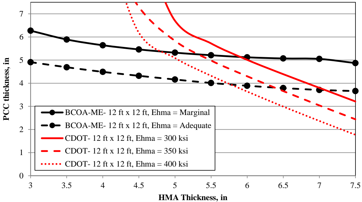
Figure 14. PCC thickness sensitivity to HMA quality for 12 ft × 12 ft slabs with respect to HMA thickness
