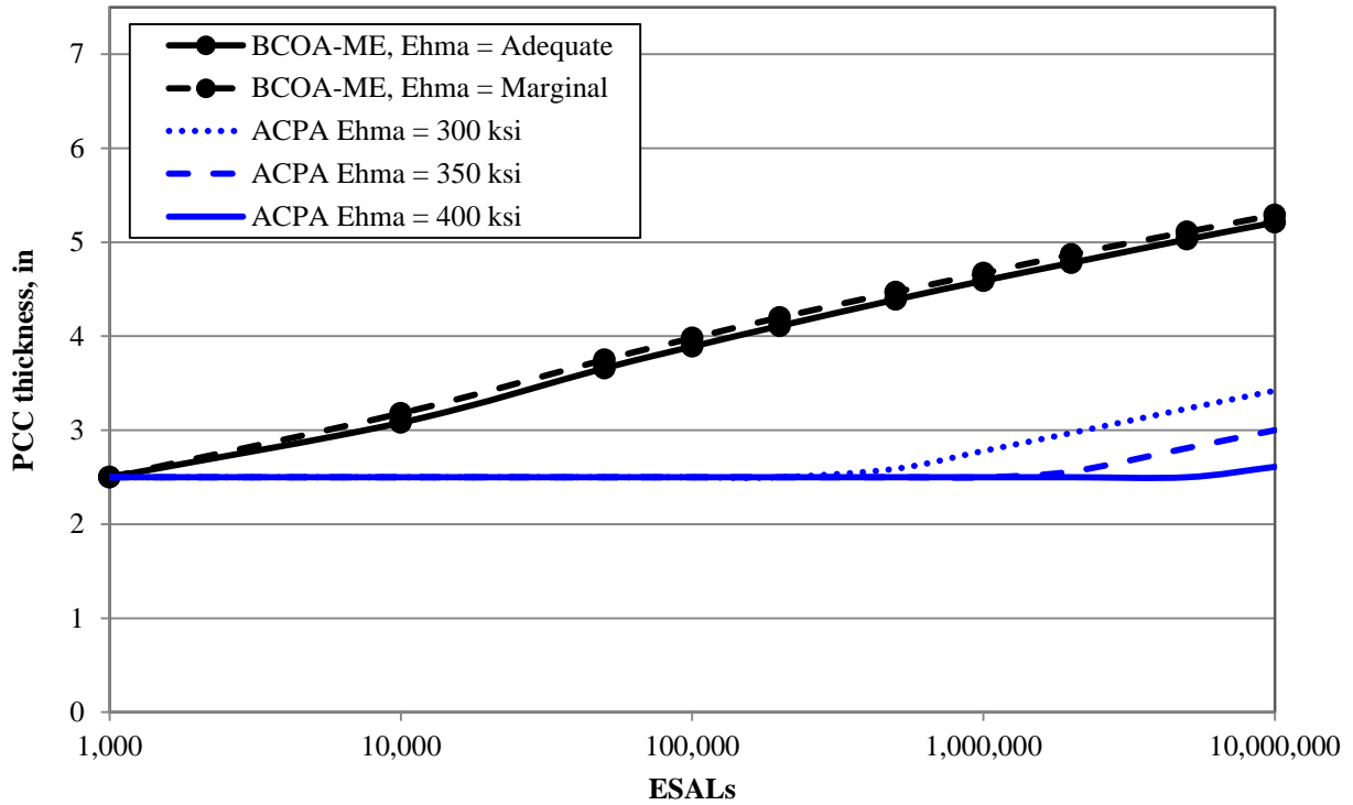
Figure 9. PCC thickness sensitivity to HMA quality for 4 ft × 4 ft slabs with respect to design ESALs
