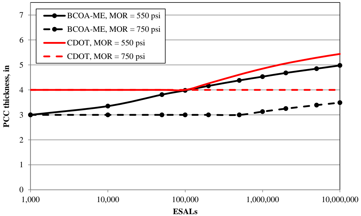
Figure 4. PCC thickness sensitivity to PCC modulus of rupture for 6 ft × 6 ft slabs with respect to design ESALs
